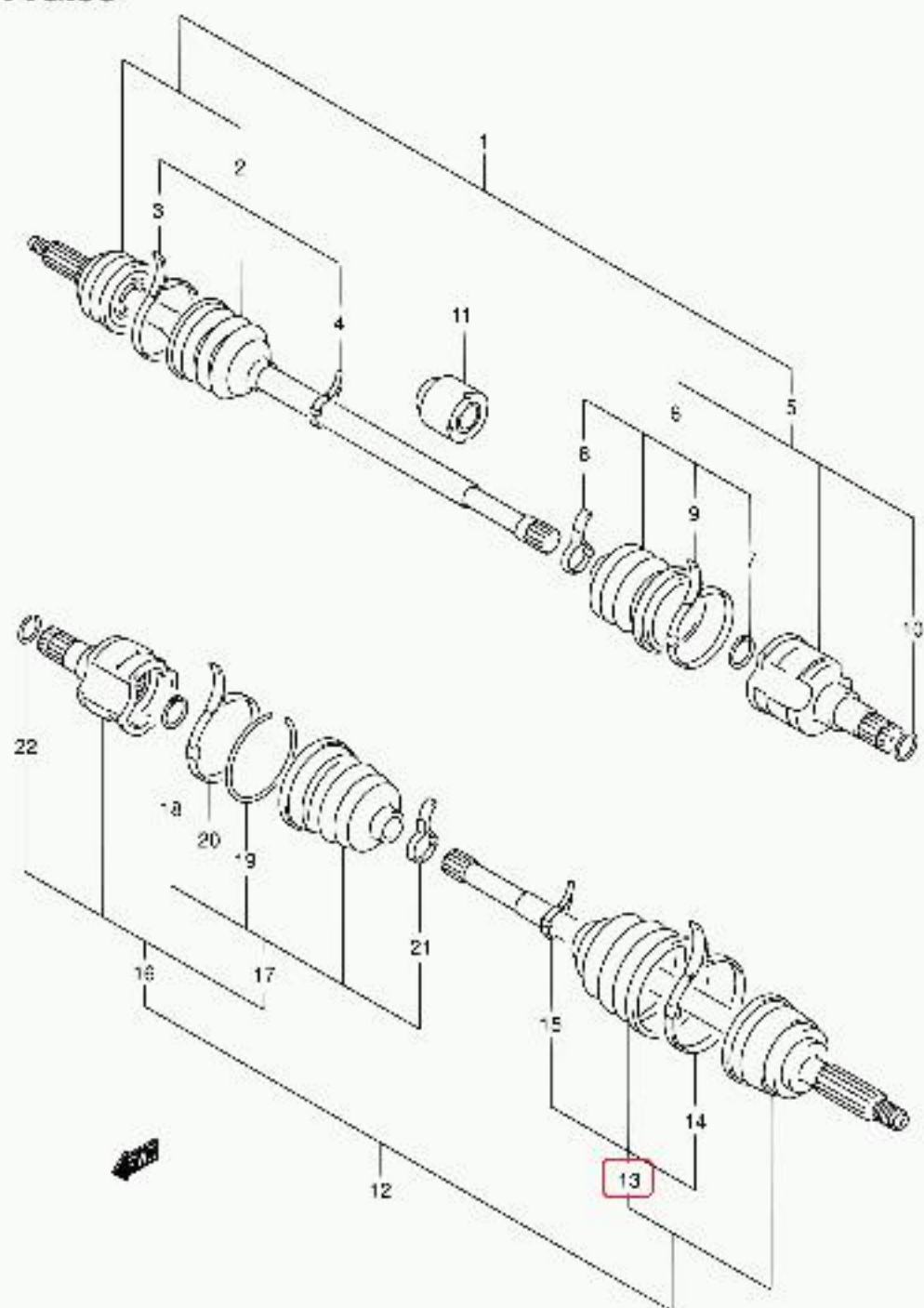
RC410 E35 058 FRONT DRIVE SHAFT(MT)
