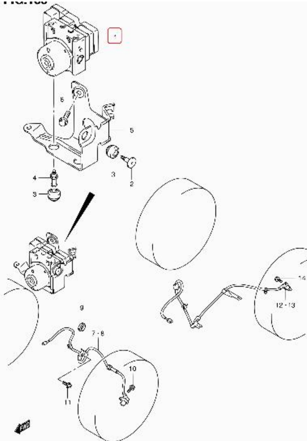
RS413 E22 168 ANTI LOCK BRAKE SYSTEM (1)
