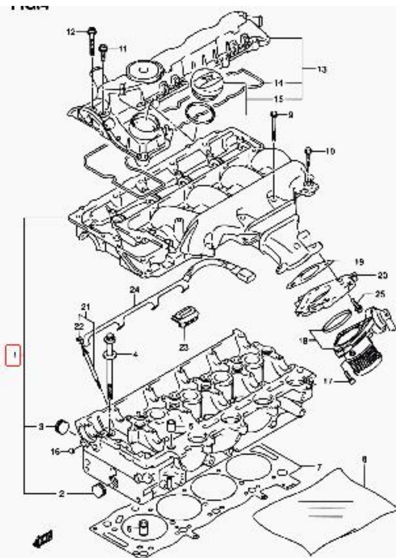
SQ420W-3 E22_504 CYLINDER HEAD (SQ420WD)
