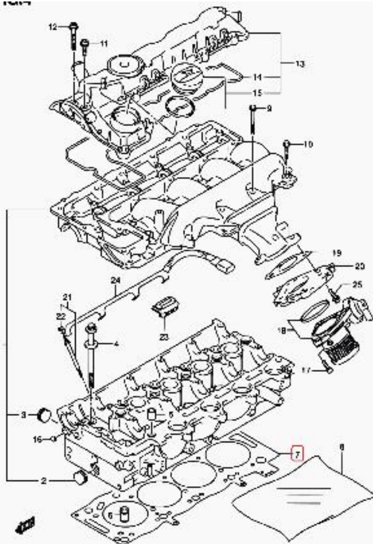
SQ420W-3 E22_504 CYLINDER HEAD (SQ420WD)
