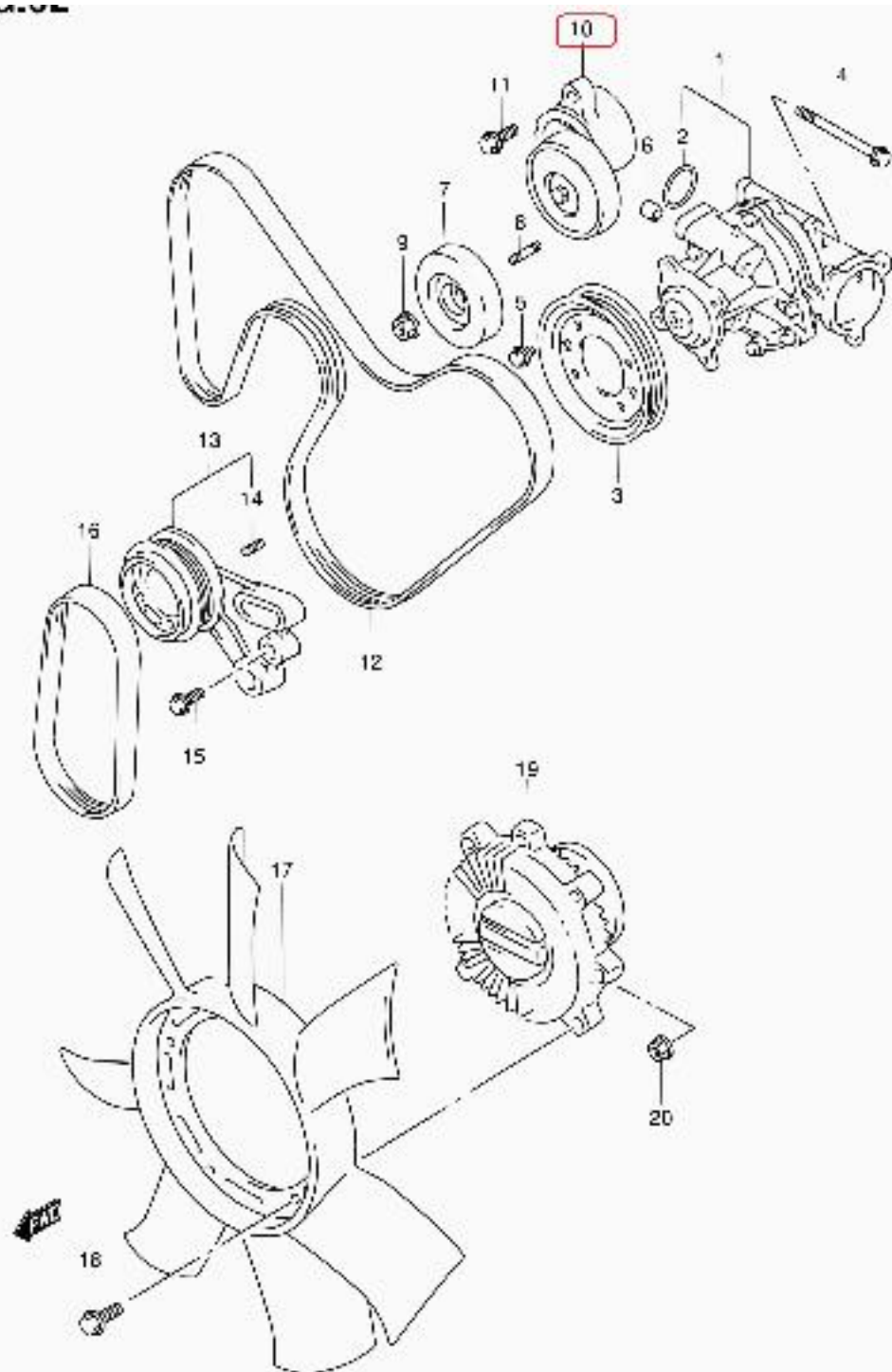
SQ416V-3 E22 062 WATER PUMP (SQ420X)
