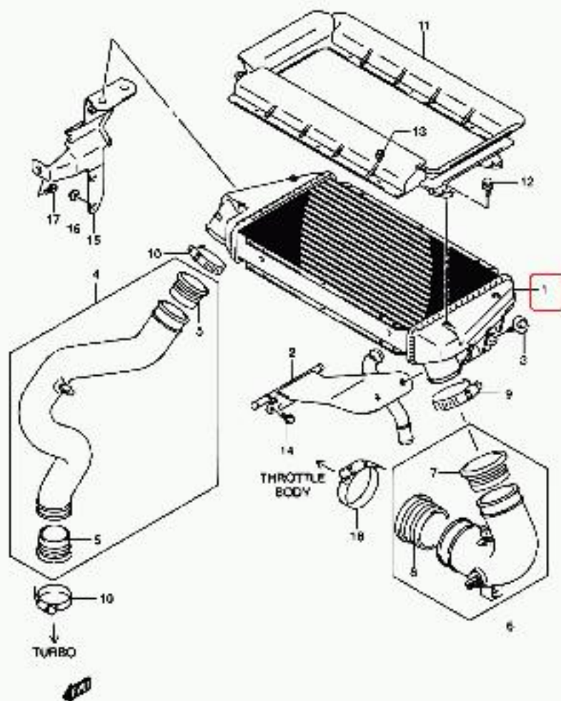
SQ420W-3 E22_009 INTER COOLER (SQ420WD)
