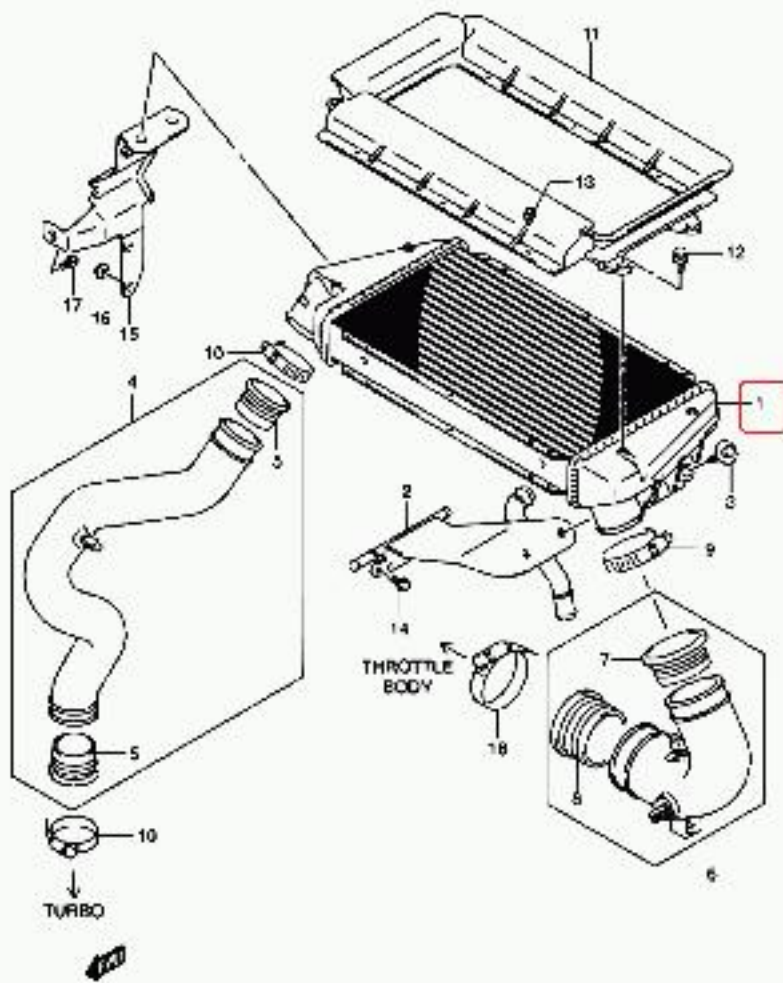
SQ420W-3 E22_019 INTER COOLER (SQ420WD)
